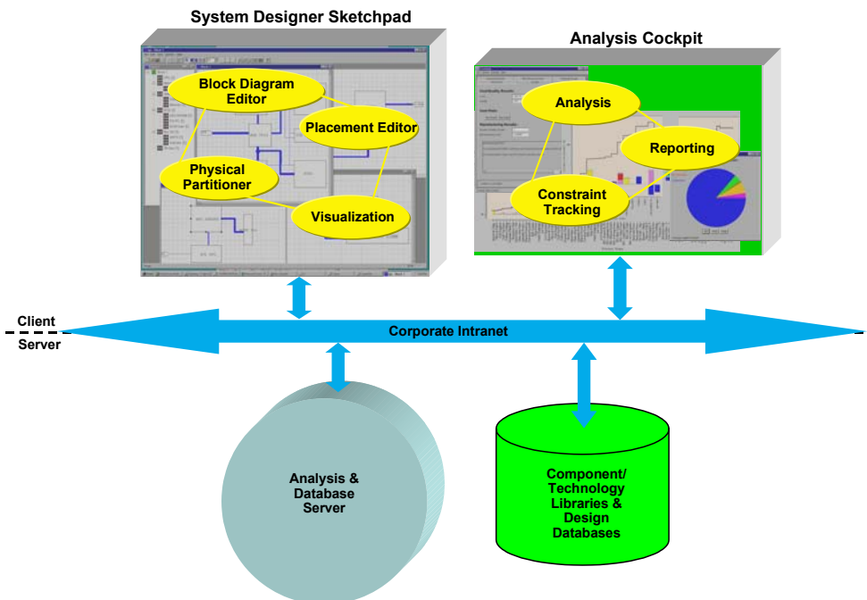
Figure 3: System Designer Sketchpad Architecture
